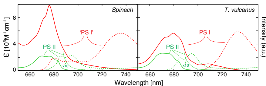
Fig. 2. Scaled absorption, solid lines & l.h. scale with corrected emission, dashed lines & r.h. scale of PS I (red) and PS II cores (green) of spinach (left panel) and T. vulcanus (right panel) at 77 K. T. vulcanus molar extinction values are room temperature values reported for Thermosynechococcus elongatus [46]. Spinach PS II extinction coefficients are taken from reported values [2] and corresponding values for spinach PS I are estimated from the integrated area of the Q_y band and scaling it to the measured chlorophyll content of the preparation (see text).
