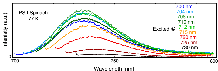
Fig. 8. Wavelength dependence of selective emission at 77 K of a spinach PS I sample (see text) excited by 70–150 mW/cm 2 laser excitation at the wavelengths indicated. Spectra are corrected for the power of the laser.
